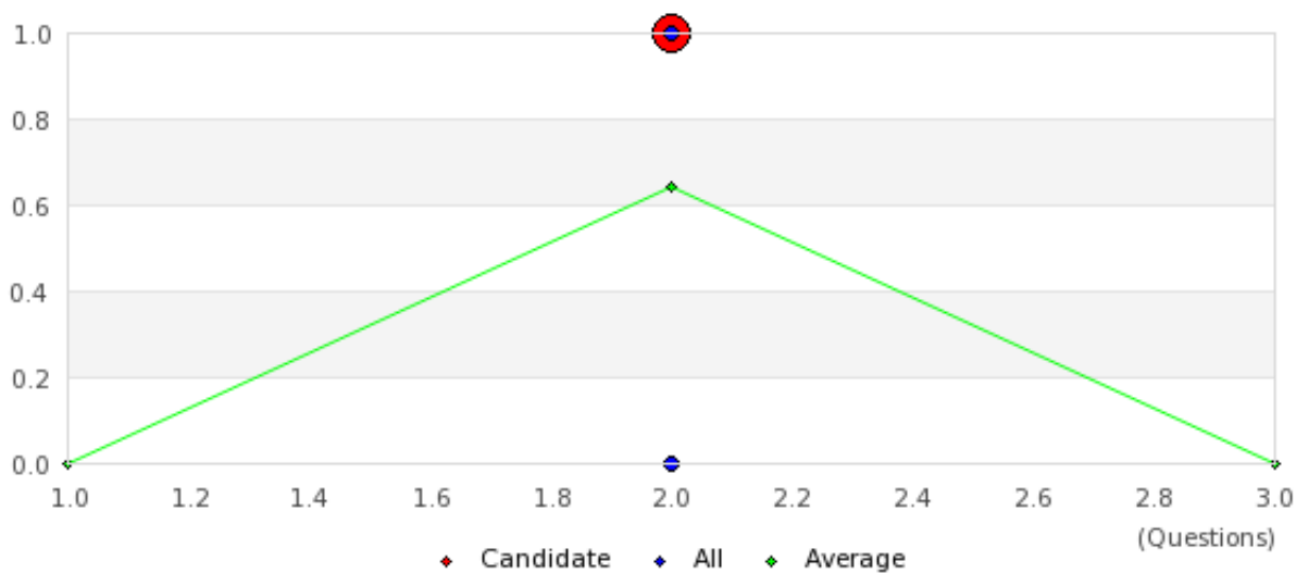
Assessment Comparison
